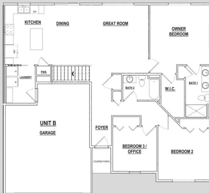
Main Level 1,583 sq. ft.
